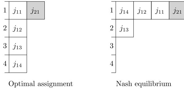
Fig. 2. Lower bound instance for m = 4, k = 2 , showing the optimal solution and a Nash equilibrium with high social cost.
