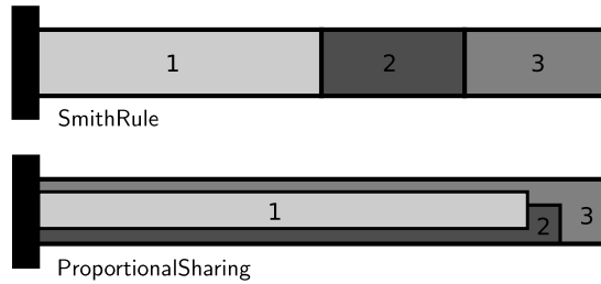
Fig. 1. Three jobs scheduled on some machine i , which uses SmithRule in the first case and ProportionalSharing in the second. Their processing times and weights are p_{i1} = 4 and w_1 = 7 for the first job, p_{i2} = 2 and w_2 = 3 for the second, and p_{i3} = 2 and w_3 = 2 for the third.
